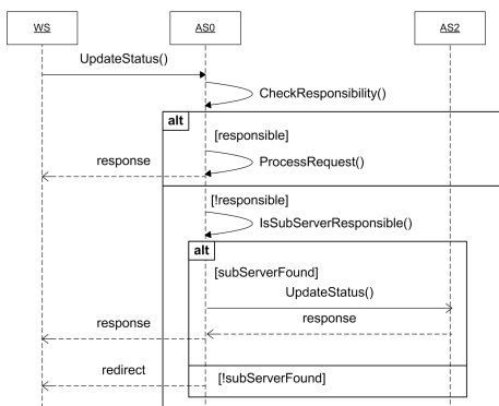
Figure 2. Selection of the responsible application server (simplified). WS is the calling web service.
